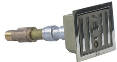
Non-Freeze Wall Hydrant with NB Box, Integral Vacuum Breaker
